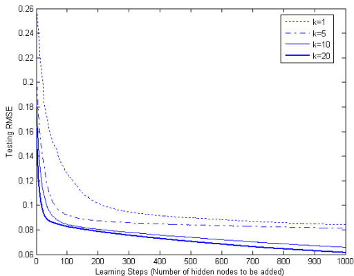
Figure 8: Testing RMSE updating progress with new hidden nodes added and different number of selecting trials k in Airplane case
