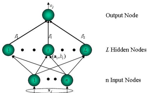
Figure 2: Feedforward Network Architecture: any type of nonlinear piecewise continuous G(\mathbf{a}_i, b_i, \mathbf{x}) .
