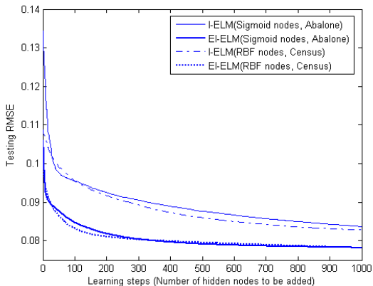
Figure 6: The testing error updating curves of EI-ELM and I-ELM
