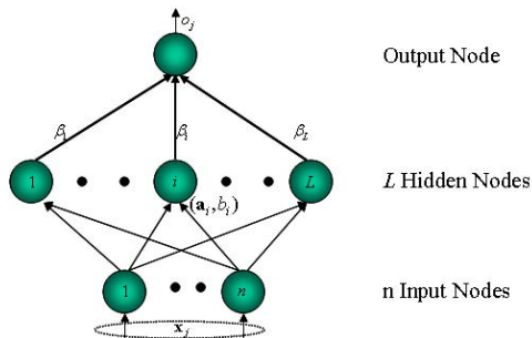
Figure 1: Feedforward Network Architecture.
