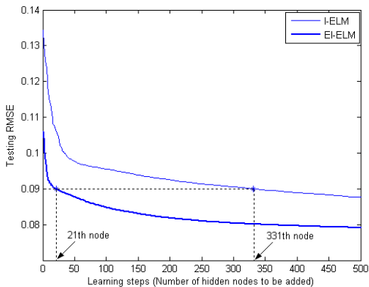
Figure 7: Testing RMSE performance comparison between EI-ELM and I-ELM (with Sigmoid hidden nodes) for Abalone case
