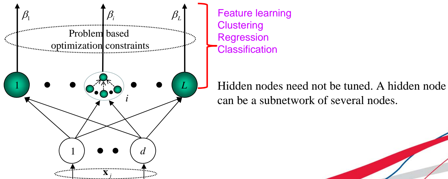
(b) ELM subnetwork
