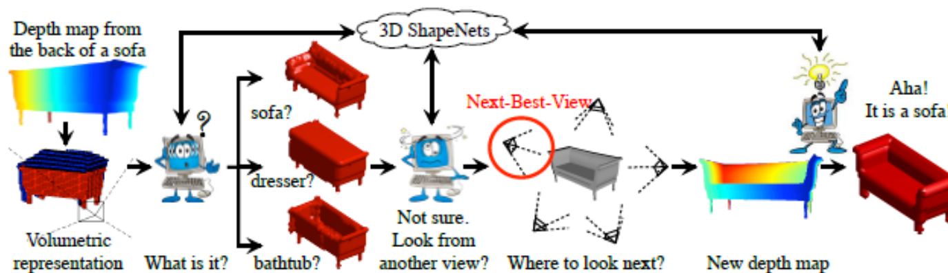
Princeton/MIT/CUHK's 3D ShapeNets for 2.5D Object Recognition and Next-Best-View Prediction [Wu, et al 2014]
