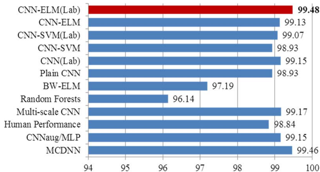
Recognition Accuracy [%]
