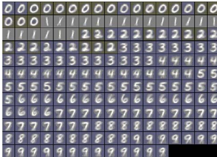
(a) ELM
