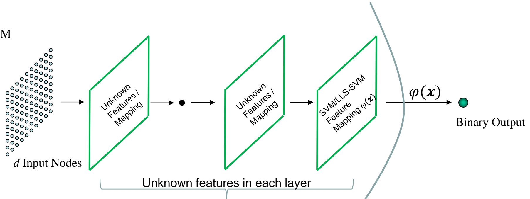
(b) Deep Learning
