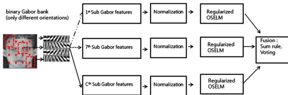
Figure 9: Binary Gabor filter-based OS-ELM (BG-OSELM)
